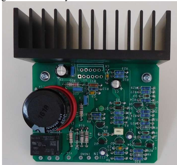
Figure 18-mounting the PCB to the heat sink
