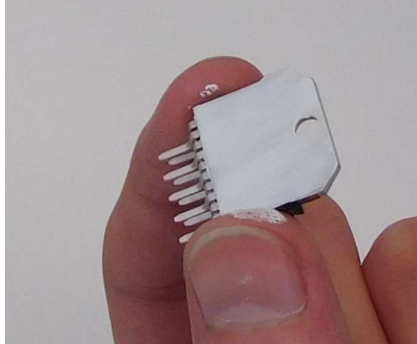
Figure 19-Spread a thin film of thermal compound on the LM3886, but keep it off the leads
