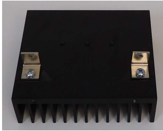
Figure 17-Mounting assembled PCB to heat sink
