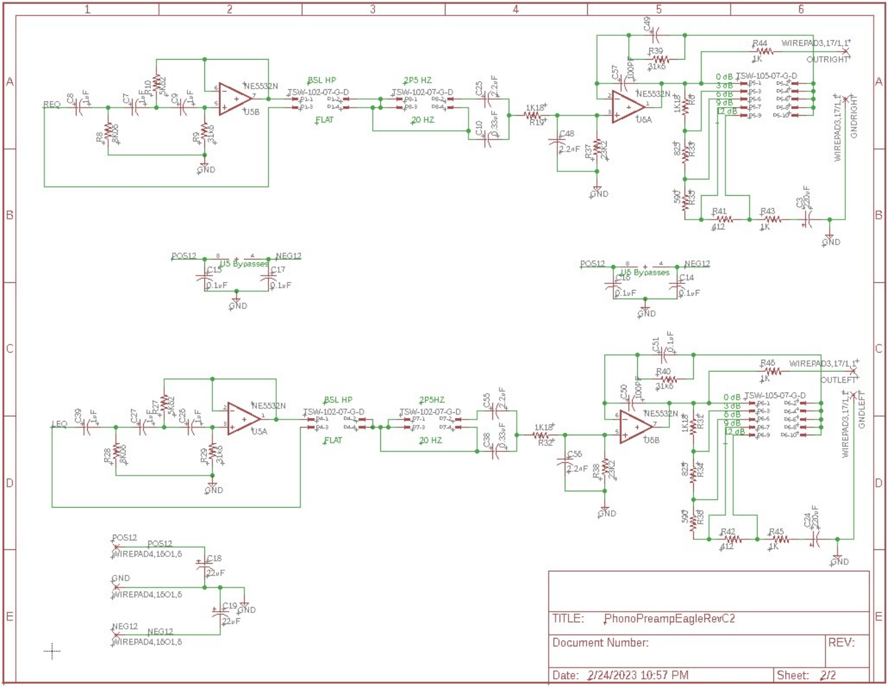
Figure 15-Schematic Page 2 of 2
